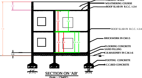
SECTION ON 'AB' (Scale :- 1"=10'0")
