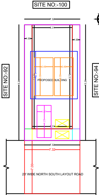
SITE PLAN
