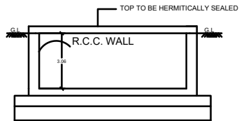
RWH SECTION (SAMPLE)
