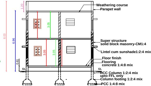
SECTION ELEVATION
