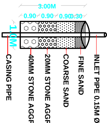
DETAILS OF RAIN WATER
