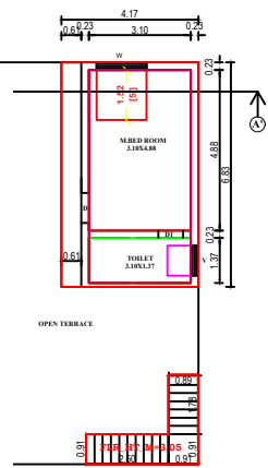
ST FLOOR PLAN
