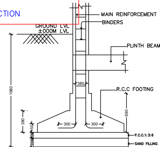
TYPICAL SECTION OF R.C.C COLUMN FOUNDATION
