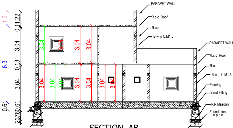
SECTION AB
