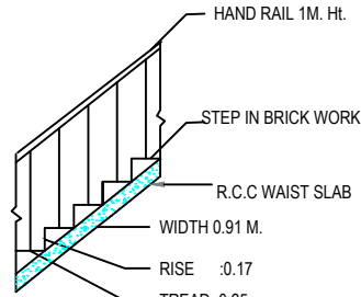
STAIR DETAIL
