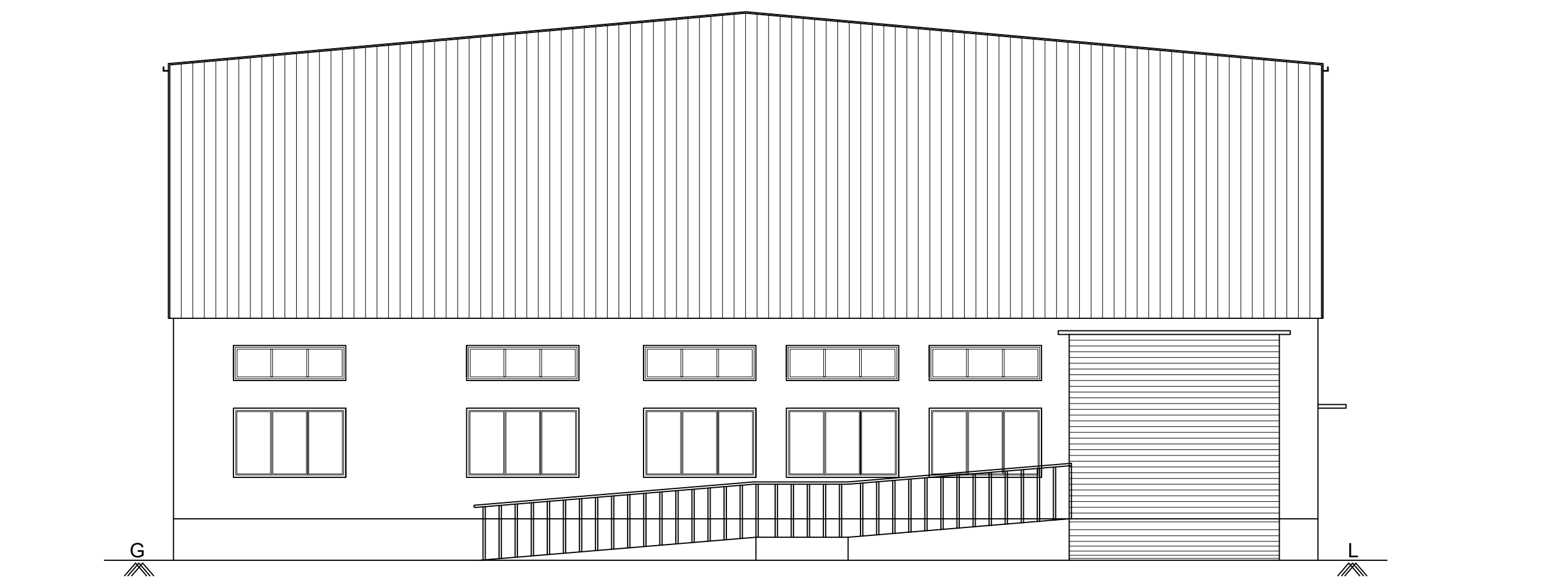
TYPICAL ELEVATION - BLOCK 1 & 2
