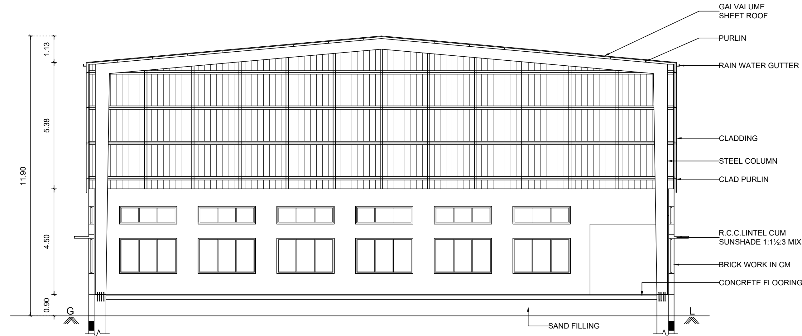
TYPICAL SECTION ON "AB" & - BLOCK 1 & 2
