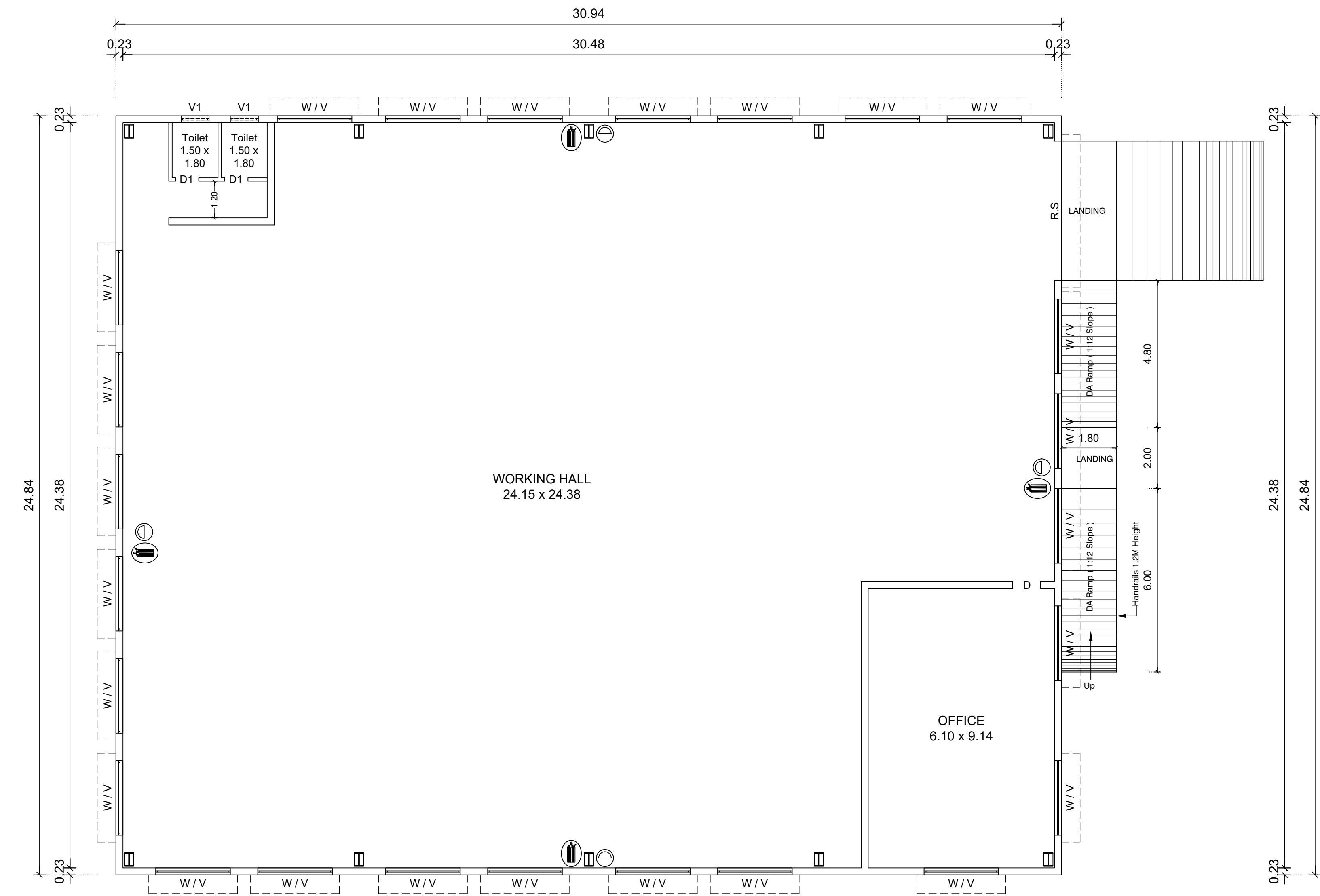
TYPICAL PLAN - BLOCK 1 & 2
