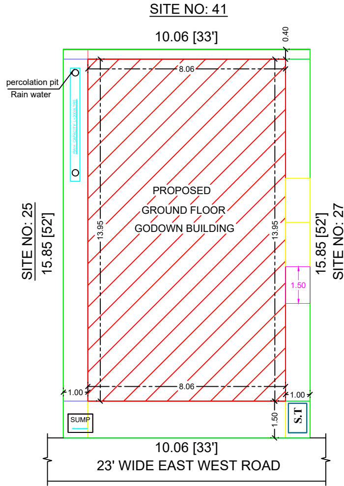
SITE PLAN
