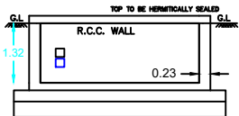
RWH SECTION
