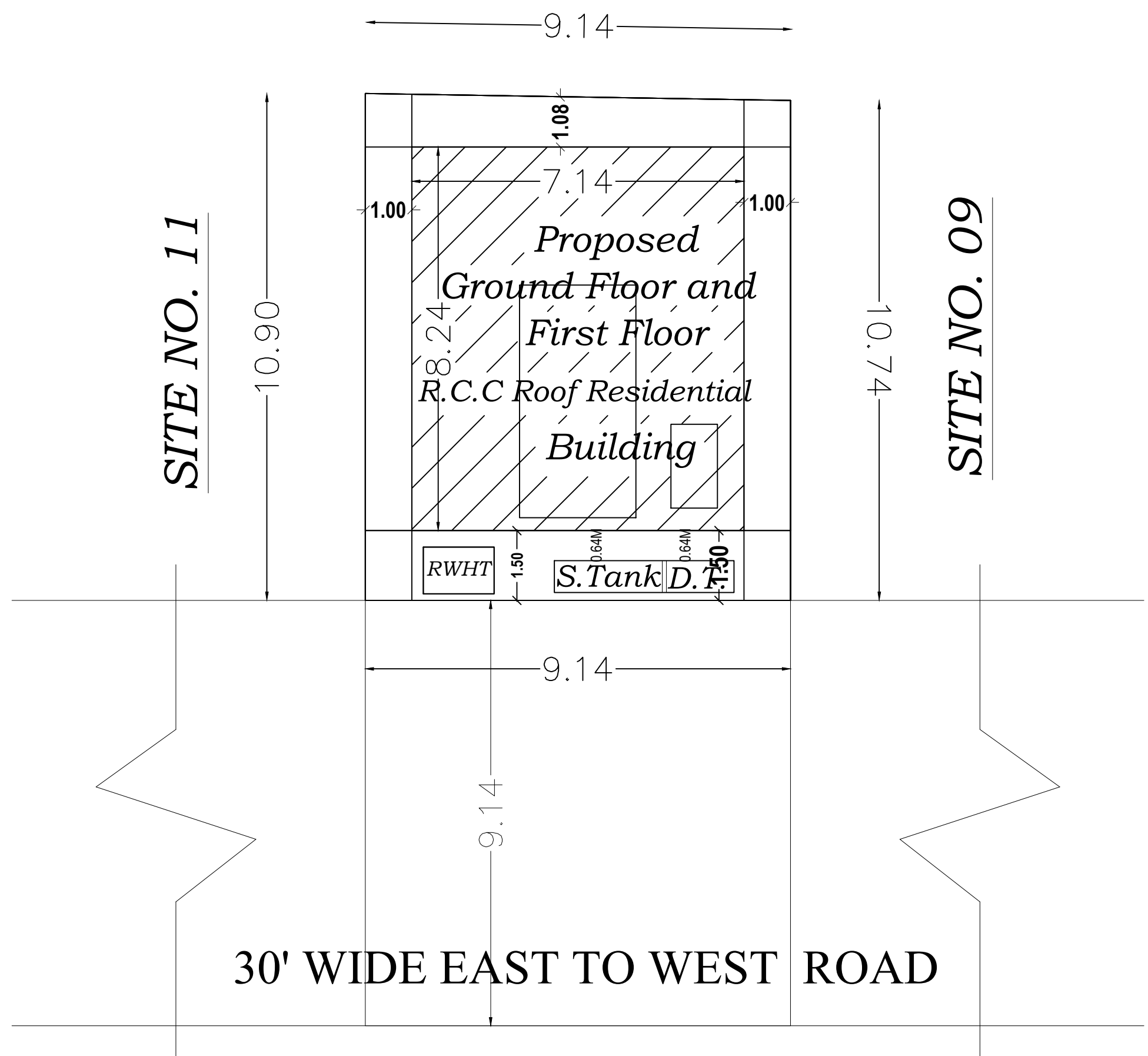
SITE PLAN
