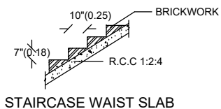
STAIRCASE WAIST SLAB
