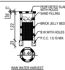
RAIN WATER HARVEST
