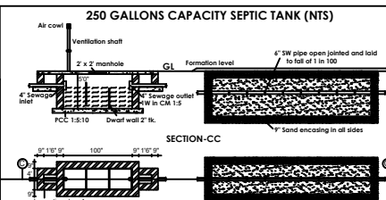
250 GALLONS CAPACITY SEPTIC TANK (NTS)
