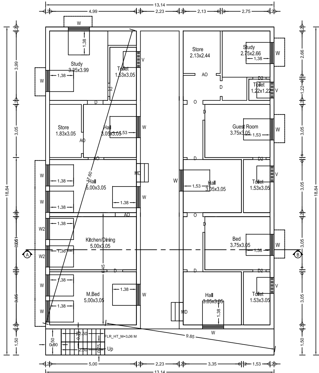
Plan Scale 1:100 Ground floor
