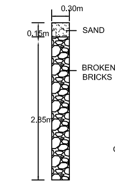
RAIN WATER HARVESTING DETAIL-PERCOLATION PIT (NTS)
