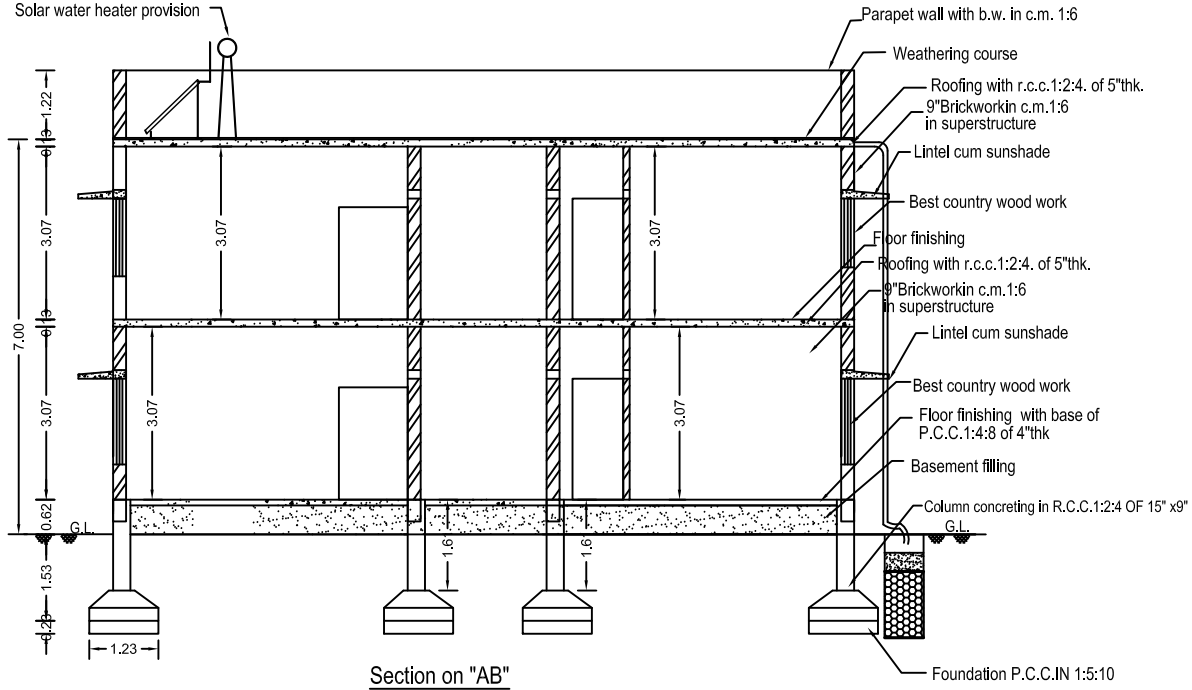
Section "AB"
