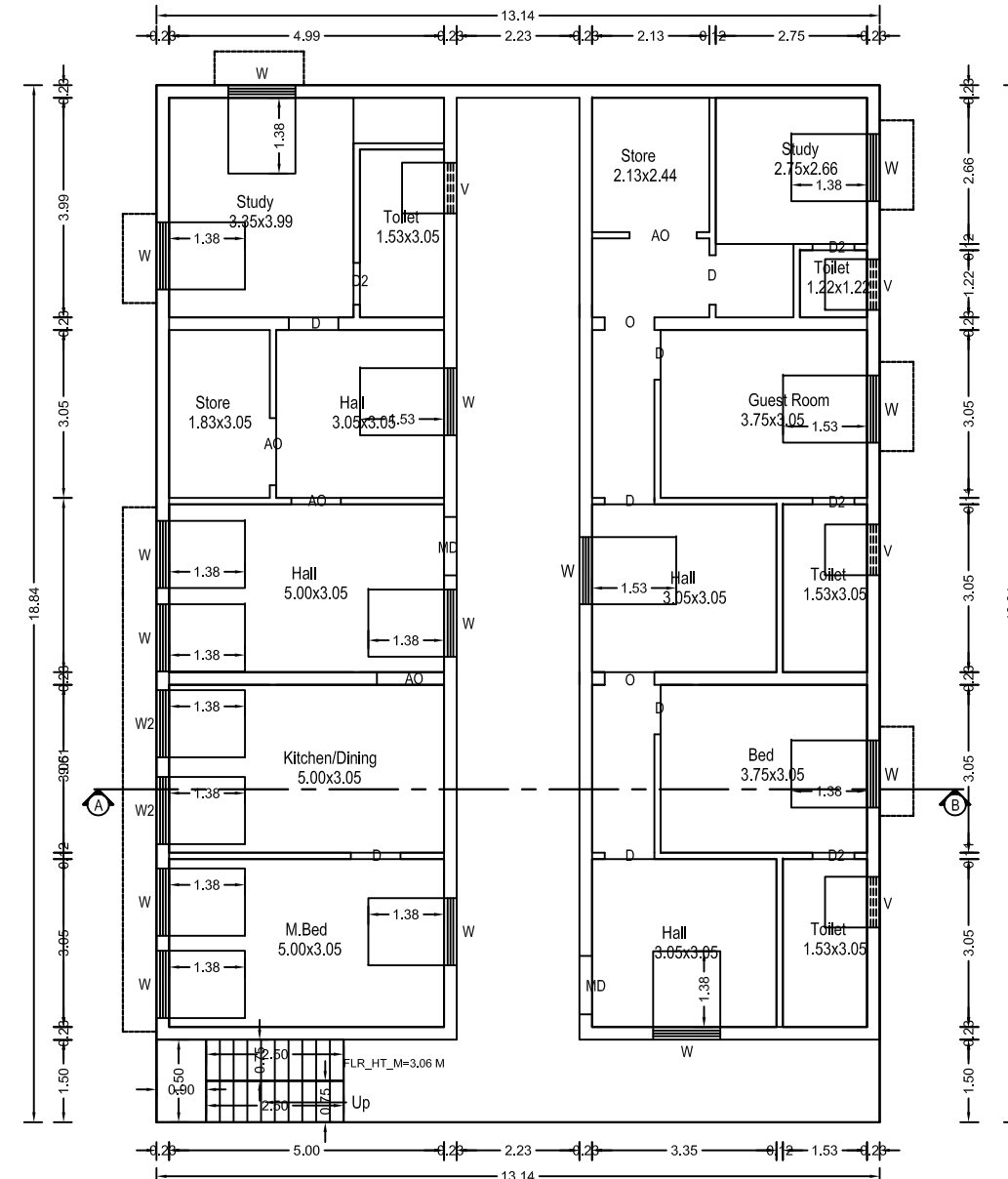
Plan Scale 1:100 First floor
