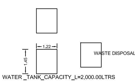
WATER_TANK_CAPACITY_L=2,000.00LTRS
