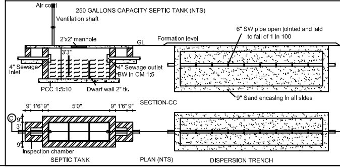
SEPTIC TANK PLAN (NTS) DISPERSION TRENCH
