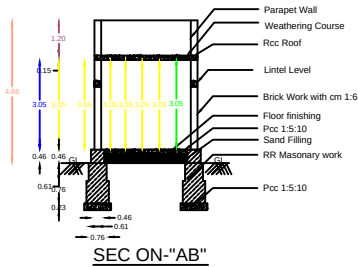
SEC ON-"AB"
