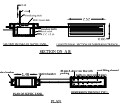
Scale Plan, Elevation, Section - 1:100
