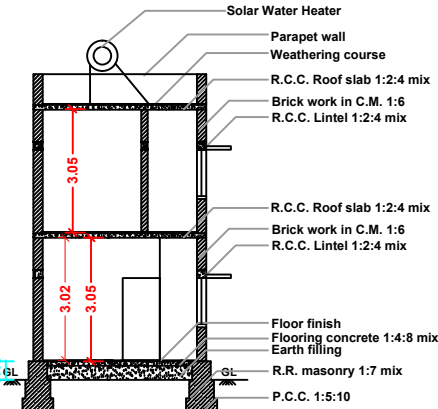
CROSS SECTION ON A-A'
