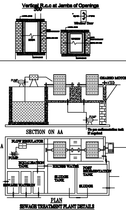
SEWAGE TREATMENT PLANT DETAILS
