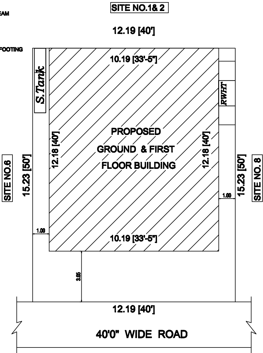
SITE PLAN
