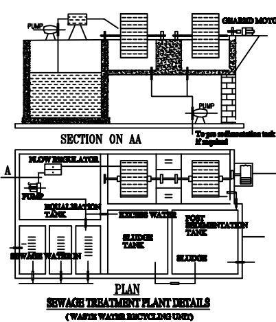
SEWAGE TREATMENT PLANT DETAILS (WATER TANK, RECTANGULAR TANK)
