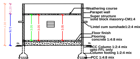
SECTION ELEVATION
