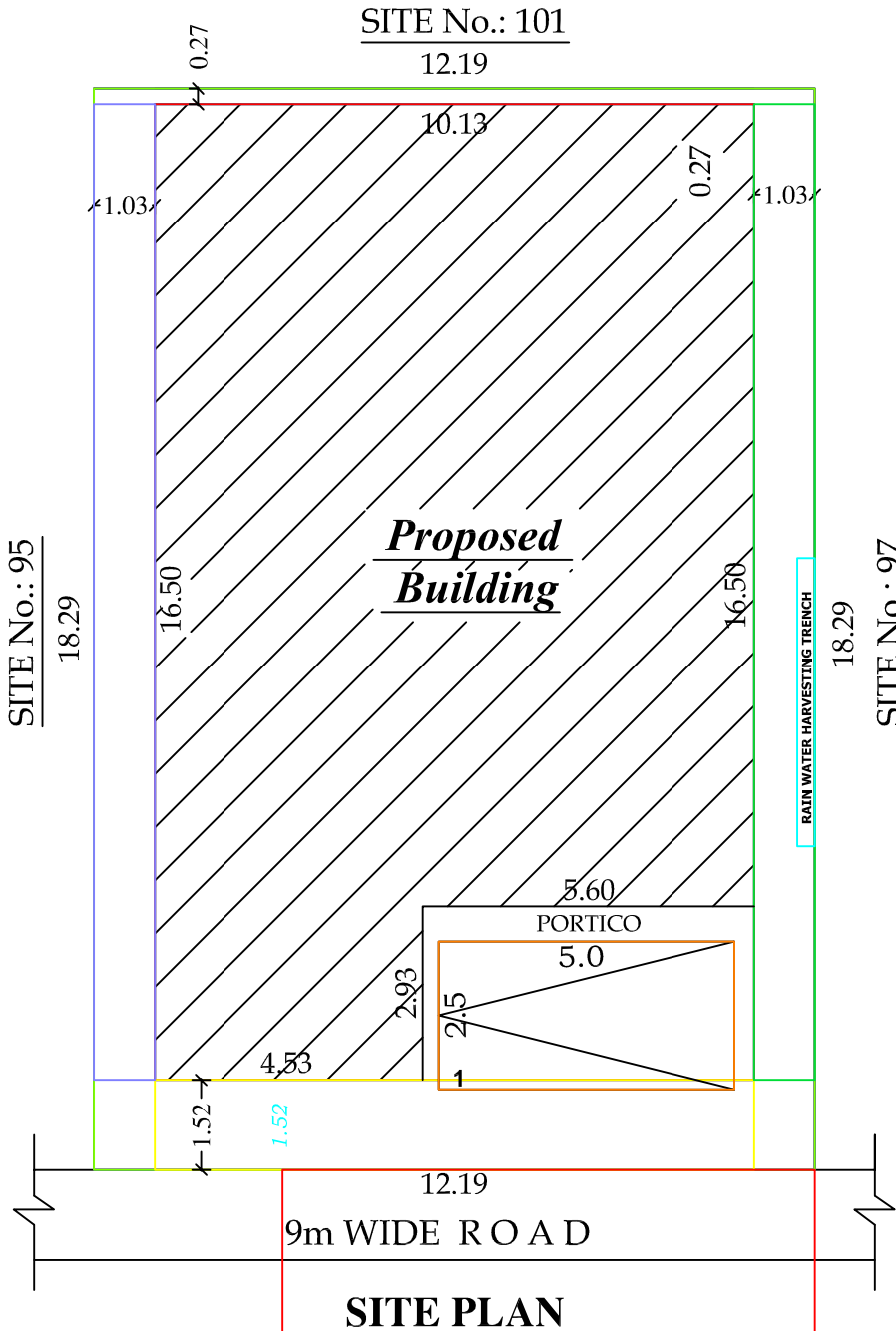
SITE PLAN
