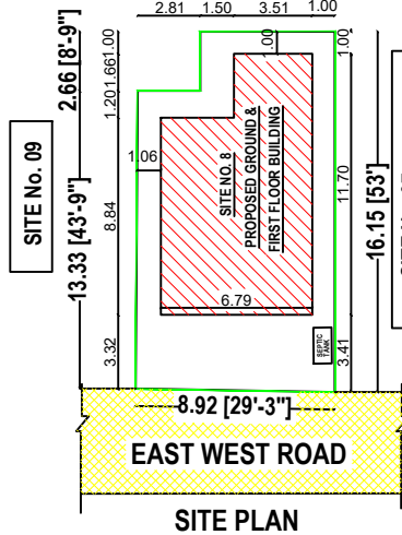
SITE PLAN
