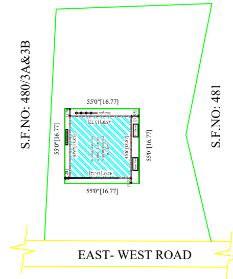
SITE PLAN
