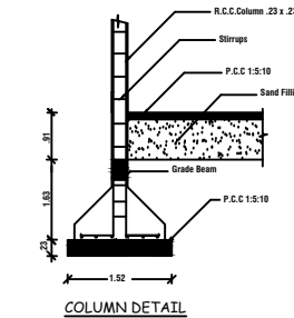
COLUMN DETAIL
