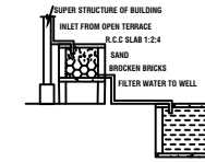
RAINWATER HARVESTING
