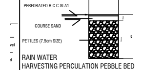
RAIN WATER HARVESTING PERCOLATION PEBBLE BED
