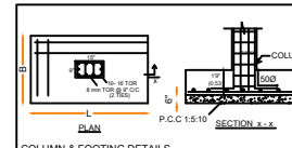
COLUMN & FOOTING DETAILS
