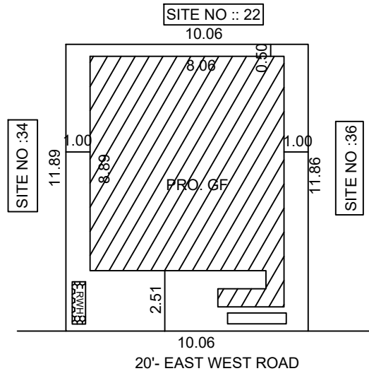
SITE PLAN
