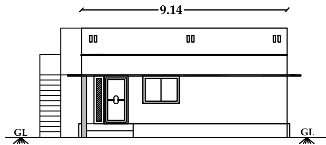
FRONT ELEVATION
