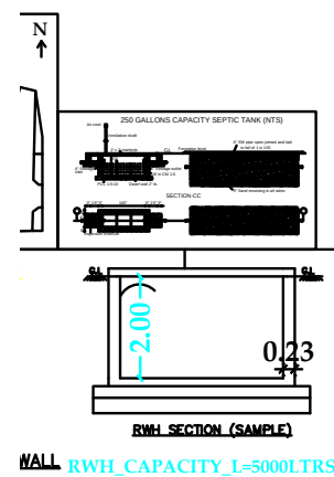
RWH SECTION (SAMPLE)
