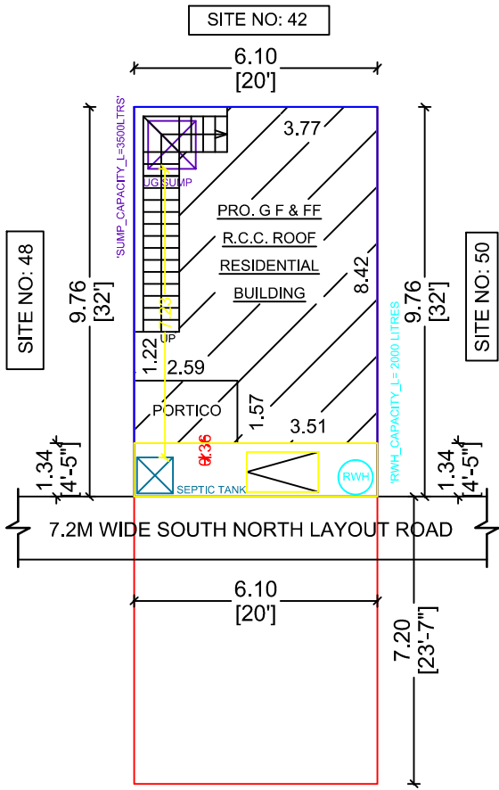
SITE PLAN
