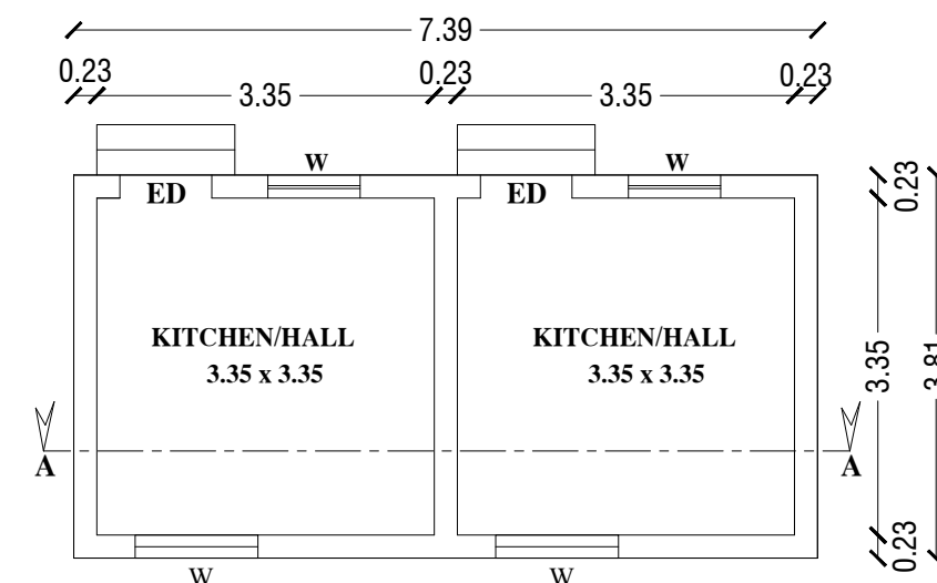
FLOOR PLAN
