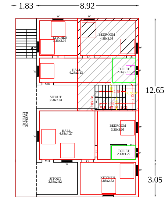
PRO.ADDL/EXISTING FIRST FLOOR PLAN
