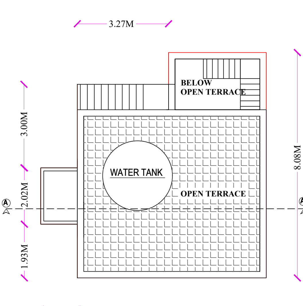
Proposed Terrace Floor Plan
