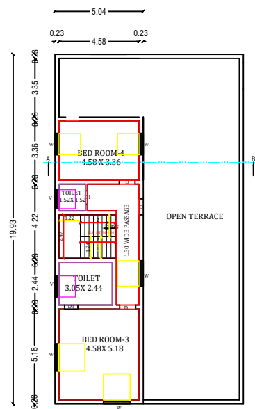
PRO.F.FLOOR PLAN
