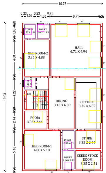
PRO.G.FLOOR PLAN
