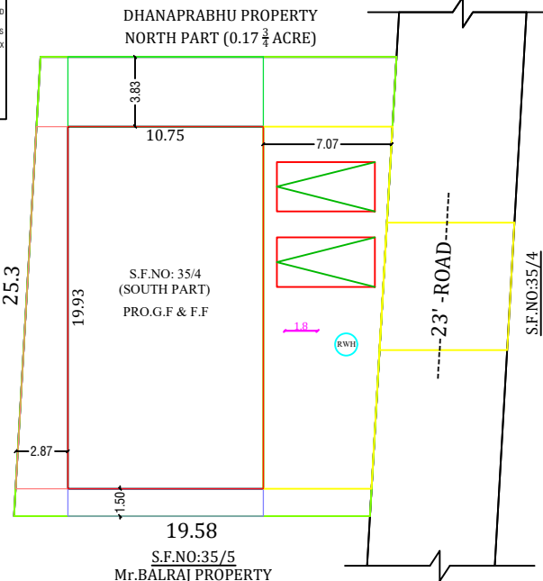
SITE PLAN
