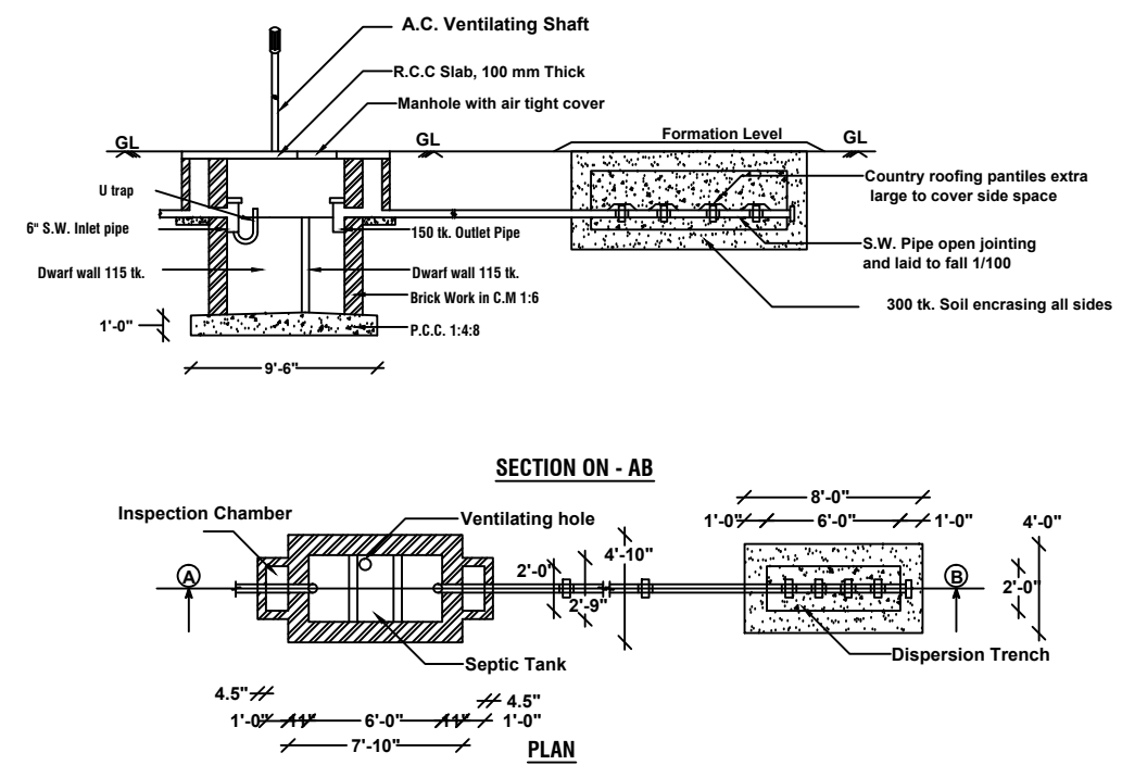
SEPTIC TANK WITH DISPERSION TRENCH ( 250 Gls.,)
