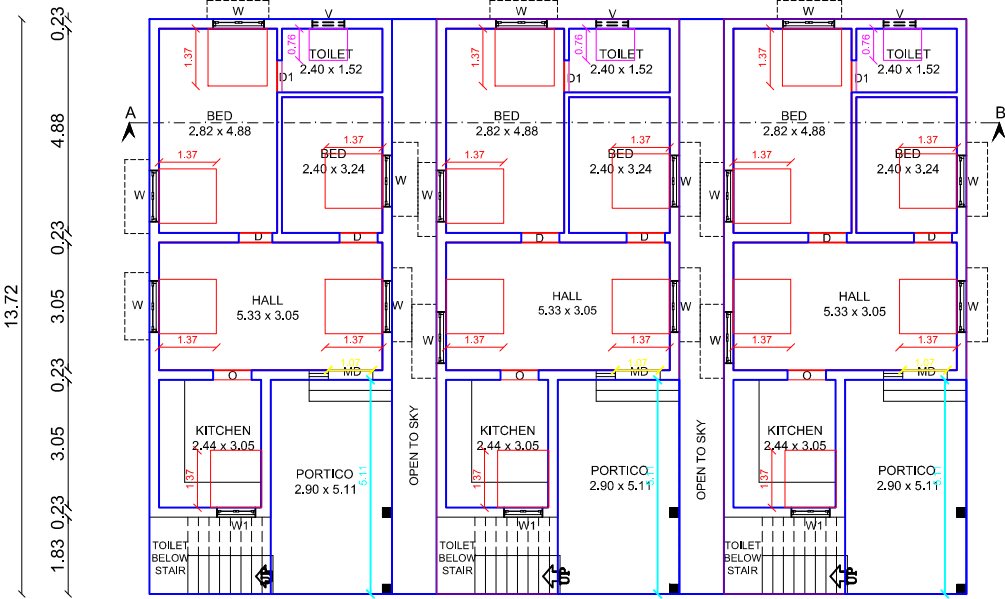
GROUND FLOOR PLAN - 1, 2 & 3
