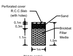
RAIN WATER HARVESTING RECHARGE TRENCH SECTION (Not to scale)
