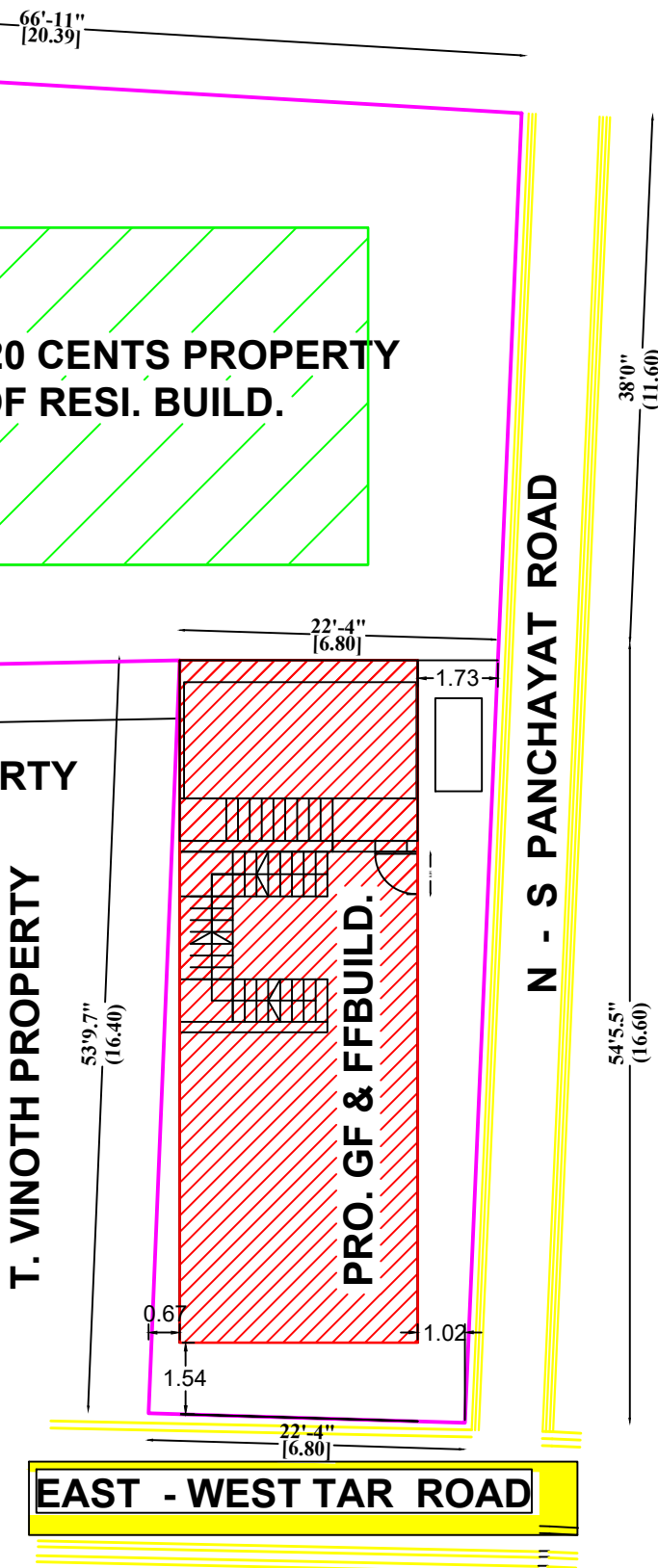
SITE PLAN
