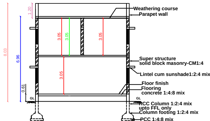
SECTION ELEVATION
