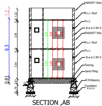
SECTION AB
