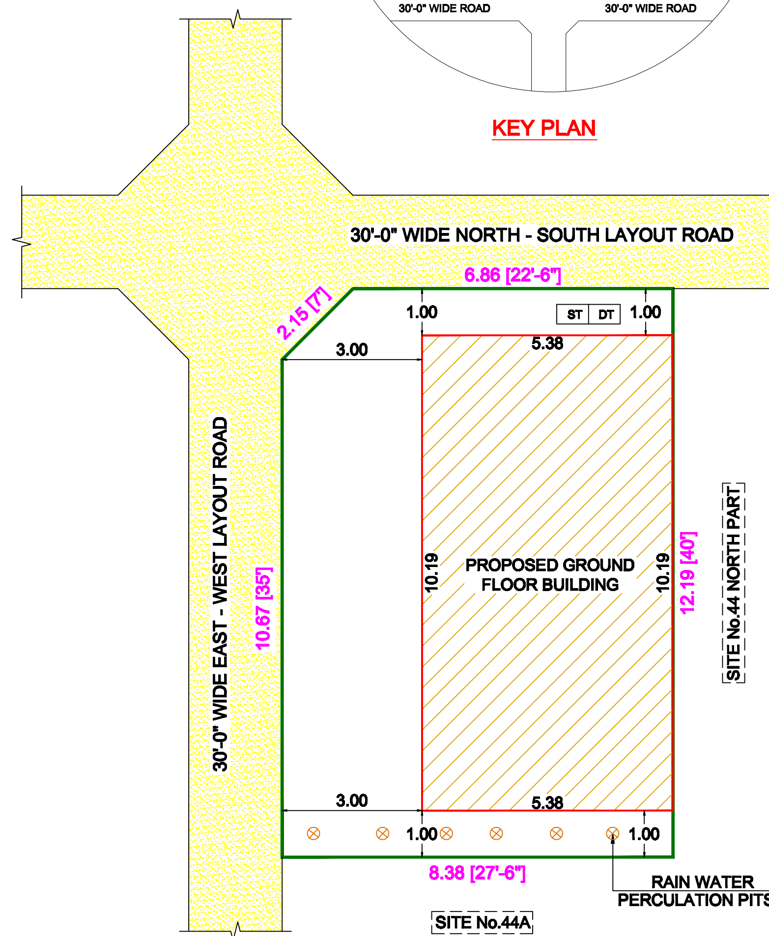
SITE PLAN
