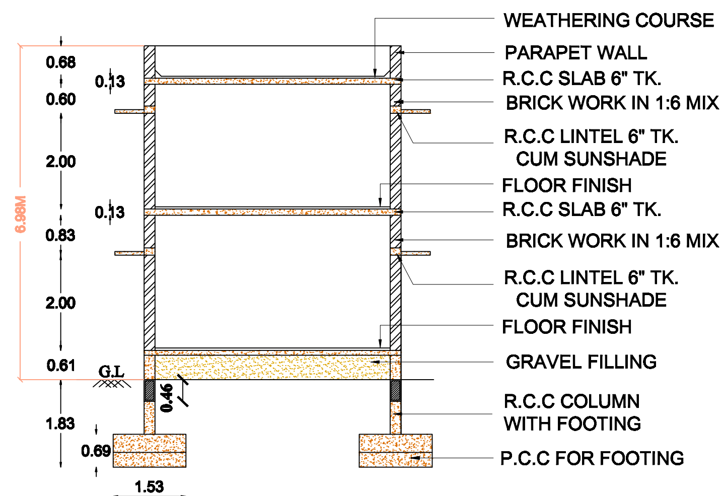
CROSS SECTION AT 'A-A'
