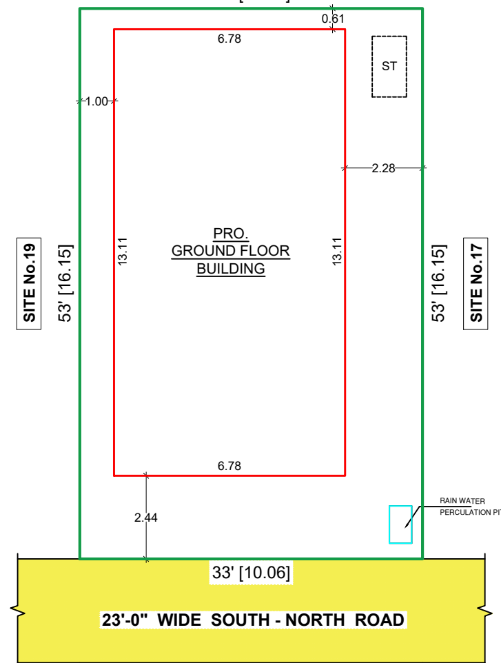
SITE PLAN
