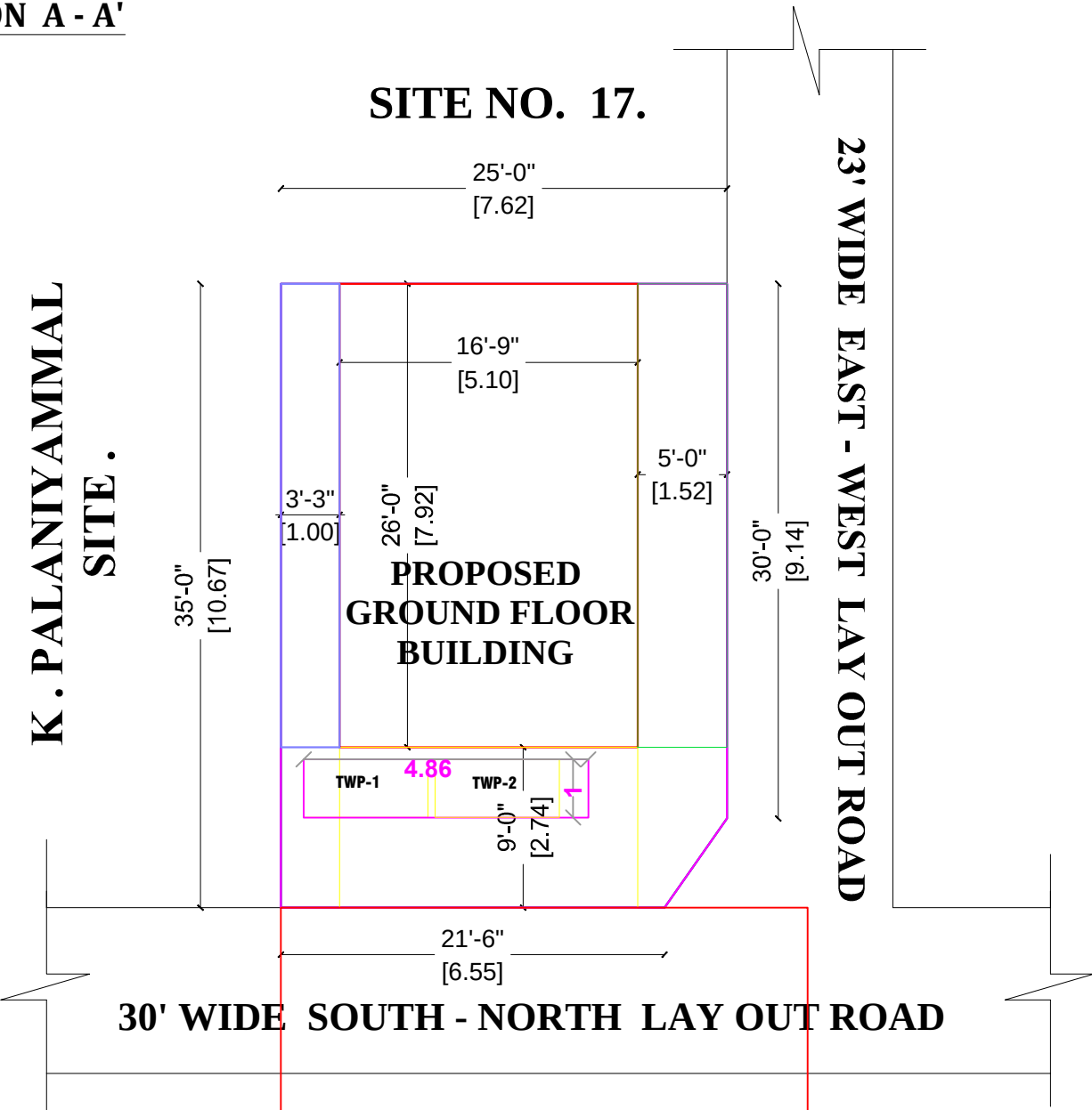
SITE PLAN
