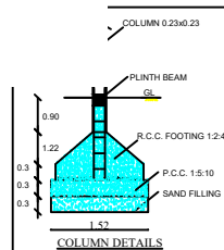
COLUMN DETAILS
