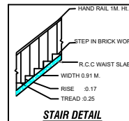
STAIR DETAIL
