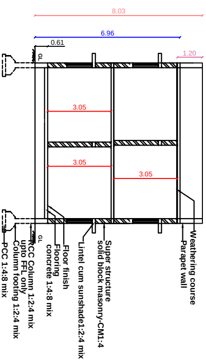
SECTION ELEVATION
