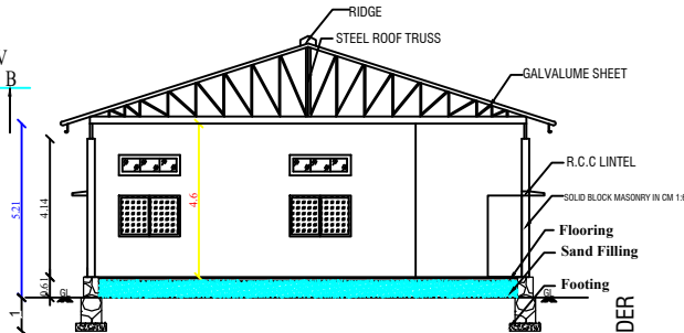
SECTION AB
