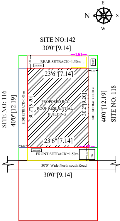
SITE PLAN
