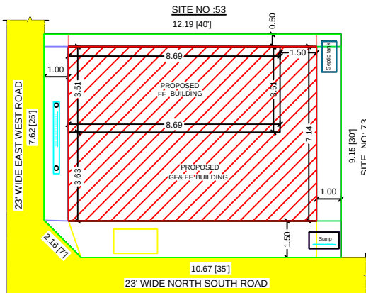
SITE PLAN
