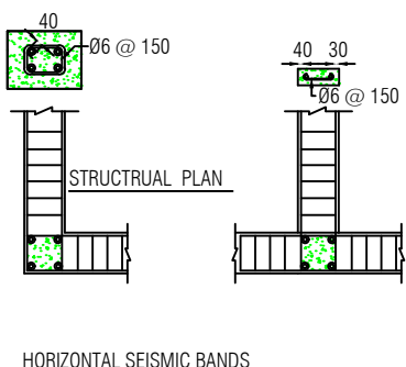
HORIZONTAL SEISMIC BANDS
