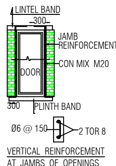
VERTICAL REINFORCEMENT AT JAMBS OF OPENINGS
