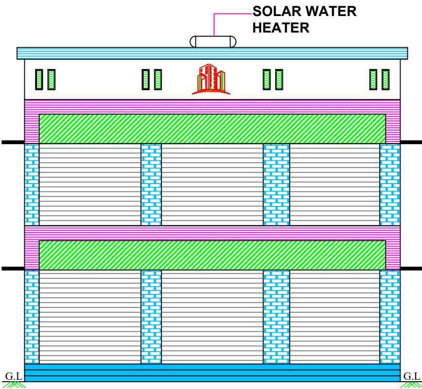
FRONT ELEVATION
