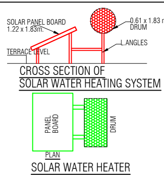
CROSS SECTION OF SOLAR WATER HEATING SYSTEM
