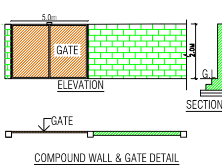
COMPOUND WALL & GATE DETAIL
