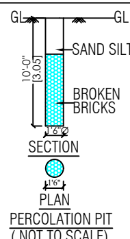
PERCOLATION PIT (NOT TO SCALE)
