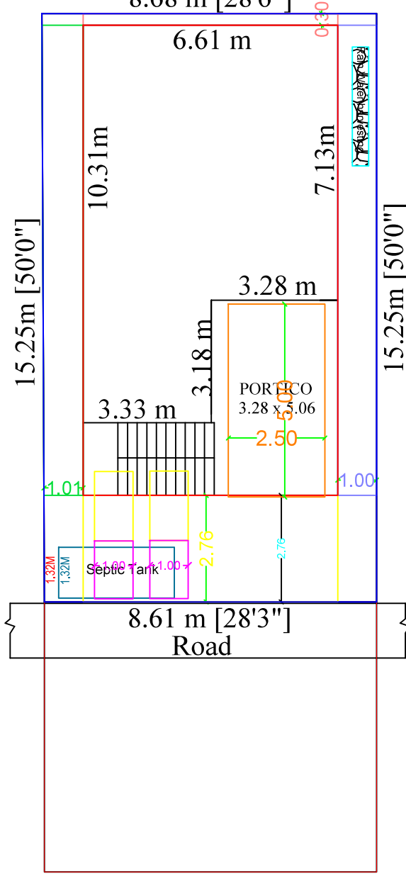
SITE PLAN [ Nts ]
