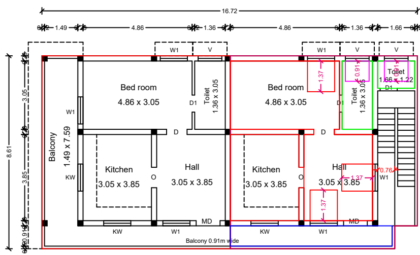
EXISTING FIRST & PRO.ADD. FLOOR
