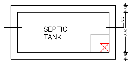
PLAN OF SEPTIC TANK SCALE 1"=2'-0"
