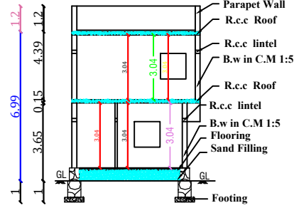
SECTION AB
