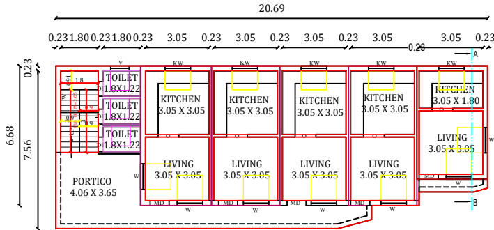
PRO.G.FLOOR PLAN
