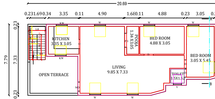
PRO.F.FLOOR PLAN
