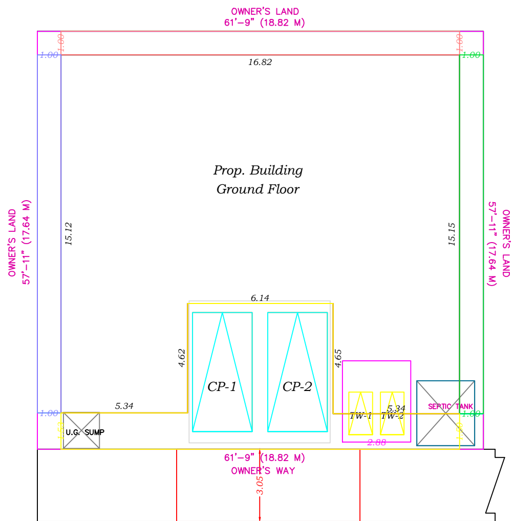
Site Plan
