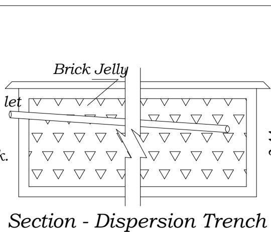
Section - Dispersion Trench
