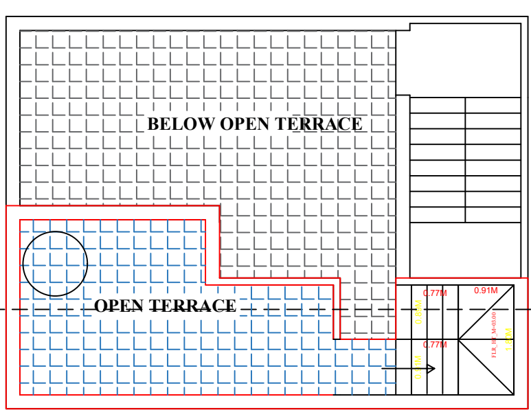
Proposed Terrace Floor Plan
